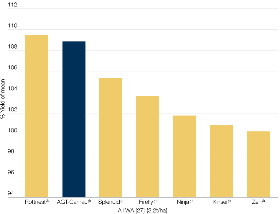
Figure 1. Grain yield of AGT-Carnac ® versus comparators across WA - AGT trials
